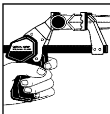
Horizontal and vertical grooves on jaw surface allow easy clamping of round stock.
